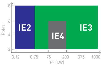
Introduction of IE4 75kW to 200kW
